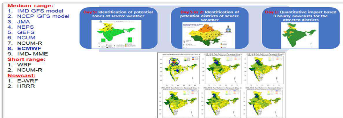
Fig 15: NWP models
