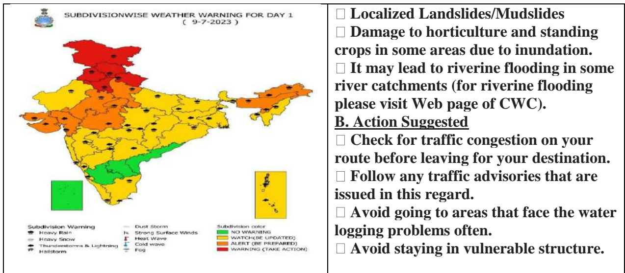
Fig 20. District wise weather warnings issued for haryana (including Chandigarh) and Punjab dated 05.07.2023
